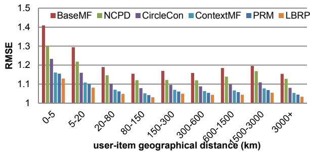
Fig. 9. The RMSE histogram in different distances based on Yelp Restaurants dataset.
