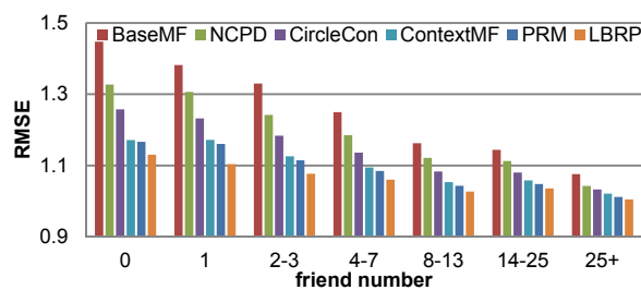
Fig. 7. The RMSE histogram of the impact of friend number.
