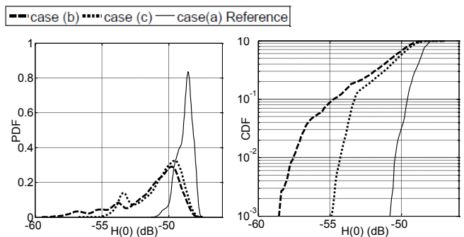
Fig. 4. H_{0-VLC} Probability Density Function and Cumulative Density Function
