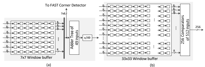
Fig. 3(a). Averaging filter (AF) of the baseline implementation, (b) Descriptor computation (DC) of the baseline implementation.
