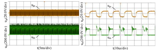
(c) Drive signal u_{gs} and drain-source voltage u_{ds} of S
