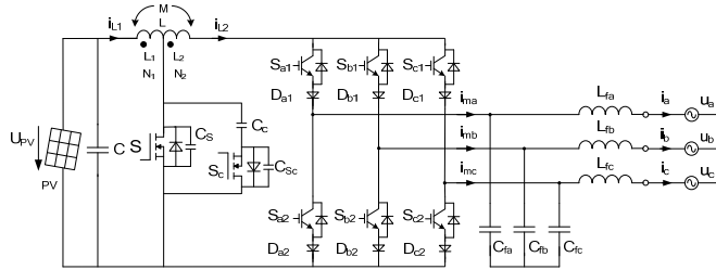
Fig. 1 Circuit topology of single-stage three-phase current-source PV grid-connected inverter with high VTR
