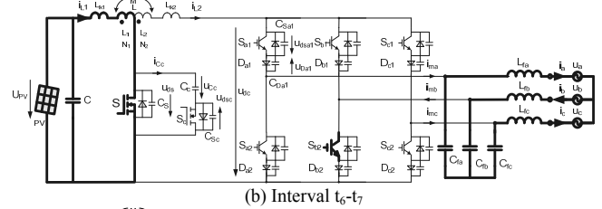
Fig. 6 HF switching process waveforms and equivalent circuits in the operating Intervals of the proposed inverter
