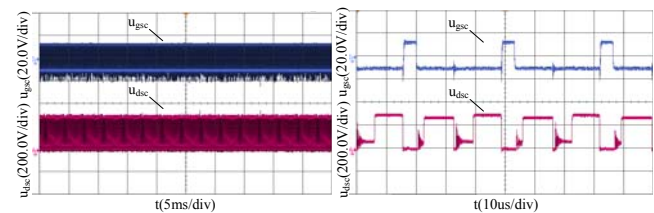
(e) Drive signal u_{gsc} and drain-source voltage u_{dsc} of S_c
