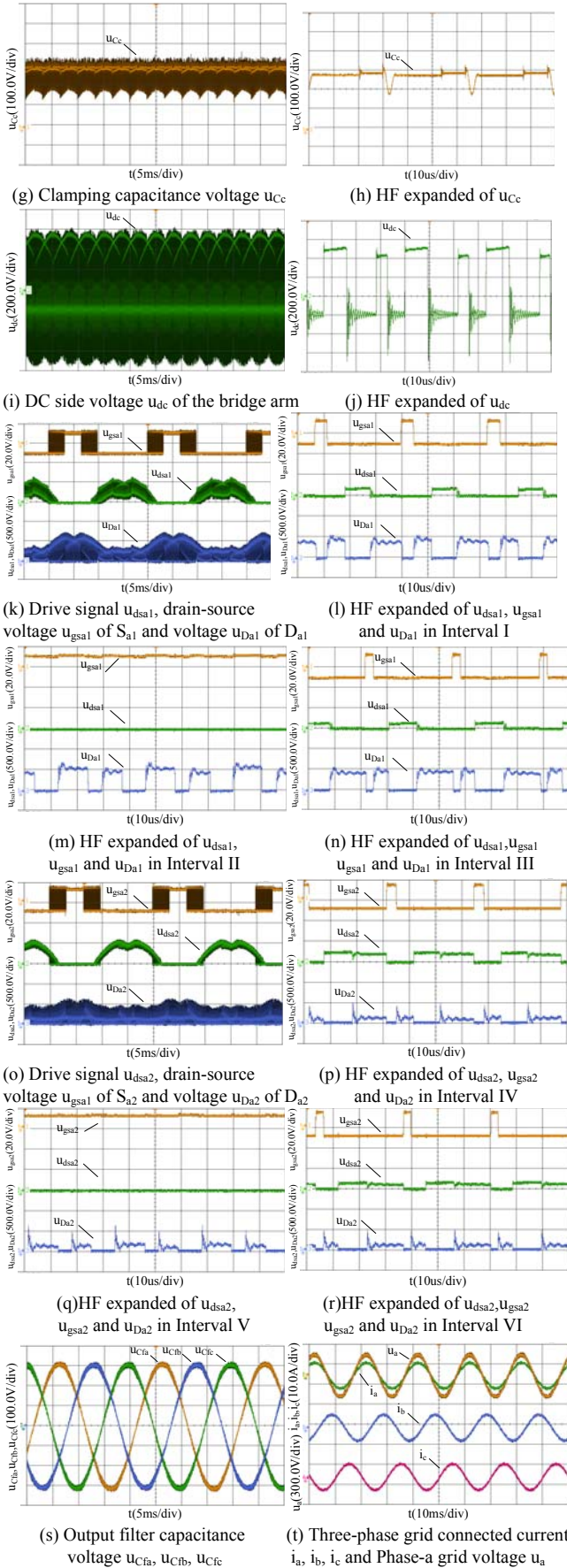
Fig. 7 Experimental waveforms of the inverter under setting MPP condition
