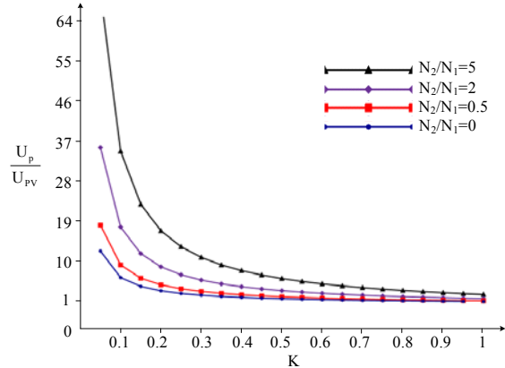
Fig. 5 Related curves between VTR of proposed inverter with coefficient K
