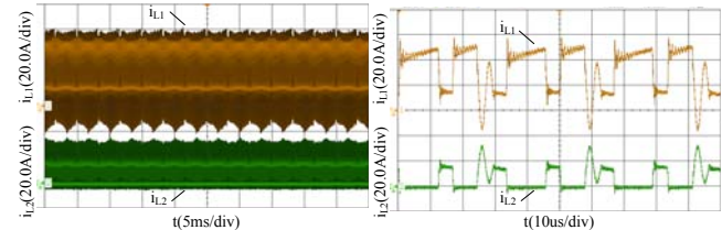
(a) Energy storage inductance current i_{L1} , i_{L2} (b) HF expanded of i_{L1} , i_{L2}
