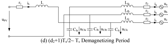
Fig. 4 Switching state equivalent circuits of the inverter in CCM mode
