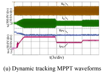
Fig. 7 Experimental waveforms of the inverter under setting MPP condition
