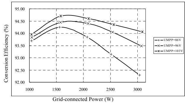
Fig. 8 Conversion efficiency curves of the proposed inverter
