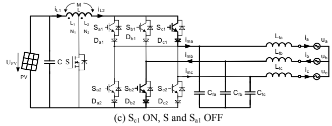
Fig. 3 Operating modes of the inverter in Interval I
