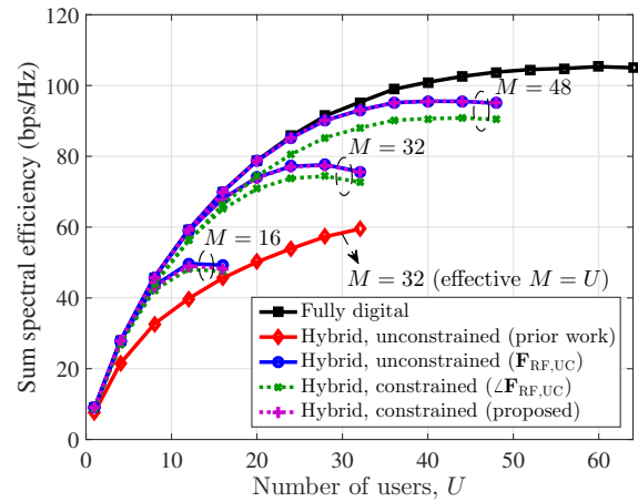
Fig. 4. Sum spectral efficiency vs. U when M \geq U , N = 64 , L = 5 , \sigma_{AS} = 10 , and SNR = 10 dB. \mathbf{F}_{RF,UC} is the proposed unconstrained analog precoder, and \angle \mathbf{F}_{RF,UC} denotes the solution of (16).
