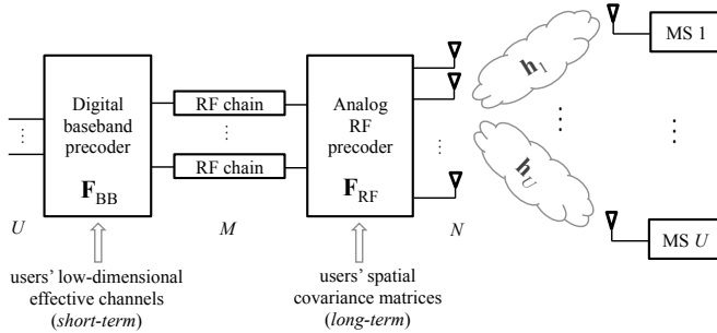
Fig. 1. Hybrid precoding for massive MIMO systems using spatial channel covariance matrices in the analog precoder design.
