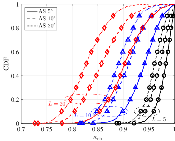
(a) CDF of \kappa_{\text{ch}} according to L and \sigma_{\text{AS}} when N = 64 , M = 32 , and U = 16 .
