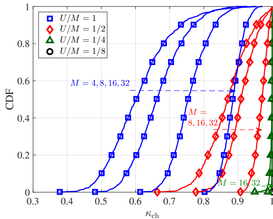
(b) CDF of \kappa_{\text{ch}} according to U and M when N = 64 , L = 5 and \sigma_{\text{AS}} = 10^\circ
