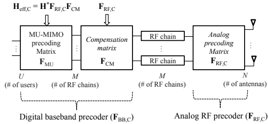
(b) Hybrid architecture for massive MIMO systems with phase shifter constraints (composed of a constrained analog precoding matrix, a compensation matrix, and a RZF baseband precoding matrix)
