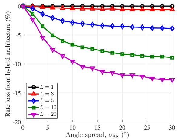
(b) Rate loss vs. \sigma_{\text{AS}}
