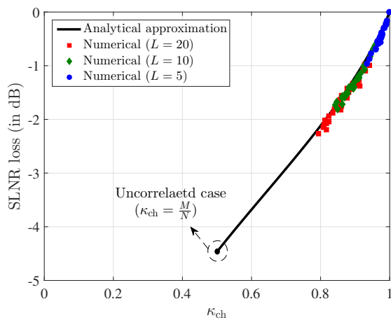
Fig. 7. SLNR gap vs. \kappa_{ch} when N = 64 , M = 32 , U = 16 , \sigma_{AS} = 10 , and SNR=10dB.
