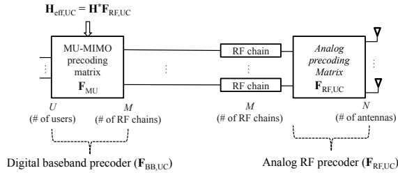
(a) Hybrid architecture for massive MIMO systems without phase shifter constraints (composed of an unconstrained analog precoding matrix and a RZF baseband precoding matrix)
