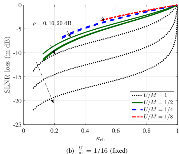
Fig. 8. SLNR gap (analytical) vs. \kappa_{ch} according to \frac{M}{N} , \frac{U}{N} , and \rho .
