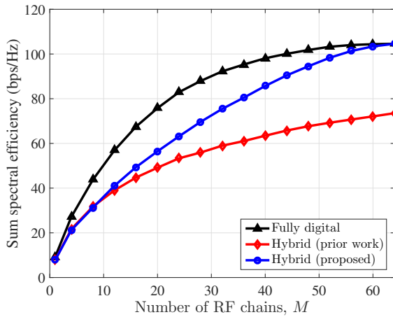
Fig. 3. Sum spectral efficiency vs. M when U = M , N = 64 , L = 5 , \sigma_{AS} = 10 , and SNR = 10 dB. Both of the hybrid precoding are performed without the phase shifter constraint. The prior work denotes the hybrid precoding technique in (2) from [16].
